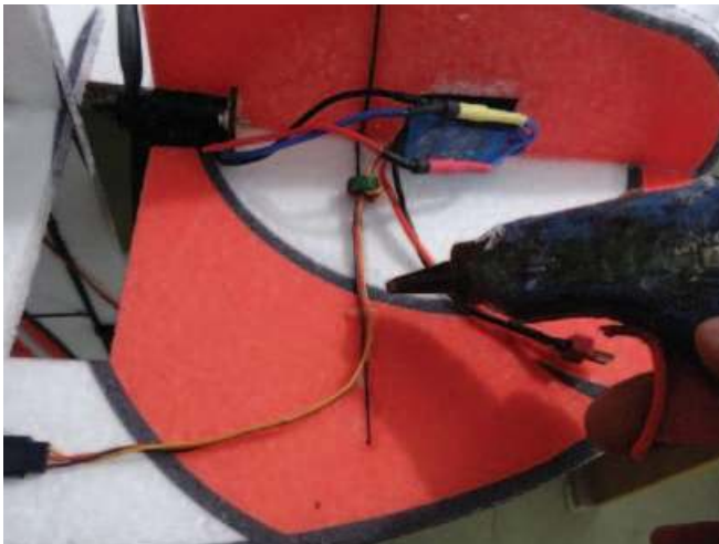
Glue the cord on carbon strip using hot glue sticks. Then connect ESC with extension cord.
