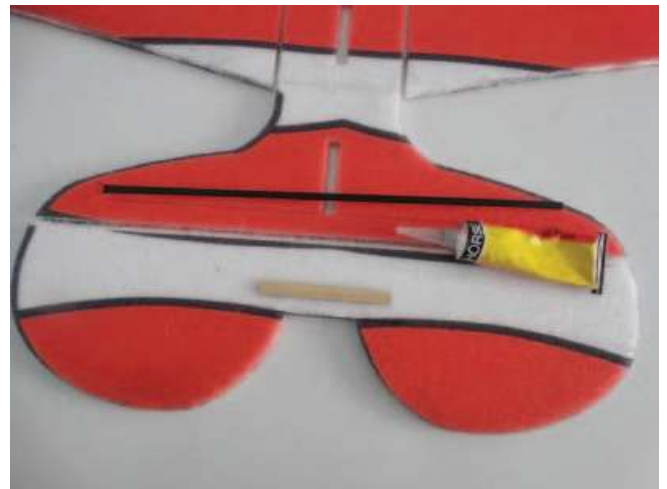
Install carbon strip and wood strip on horizontal tail using foam glue. Then wait glue dried.
