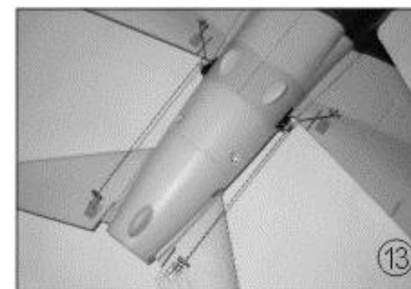
Fig. 13 - Photo shows the finished view after the skids are assembled.
