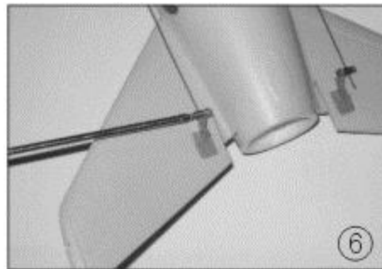
Fig. 6 - Tight the set screws on the elevator EZ connectors. elevator steel wire with cross screw and trim lever.
