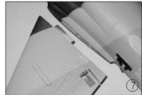
Fig. 7 - Apply glue to the sides of each main wing panel (glue not included).
