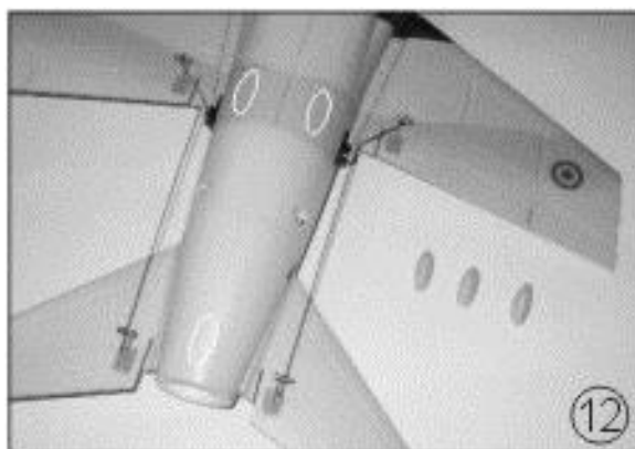
Fig. 12 - Locate the landing skids and apply glue to the back of the fuselage. (white mark shows the
