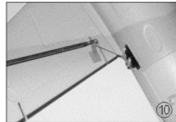
Fig. 10 - Connect the push rods to the aileron servo arm and trim lever control horns.
