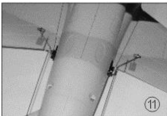
Fig. 11 - Photo shows the finished view after all steel wires assembled.
