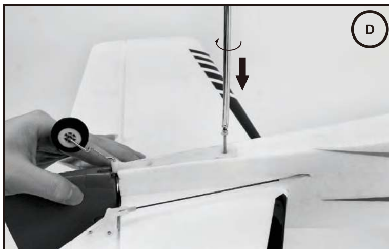
2 x Screw 2.6 x 35mm
